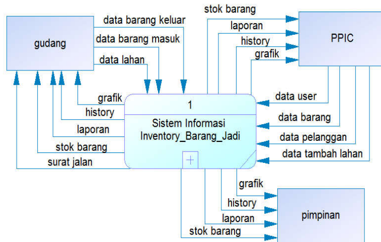
Figure 3 Context Flow Diagram
