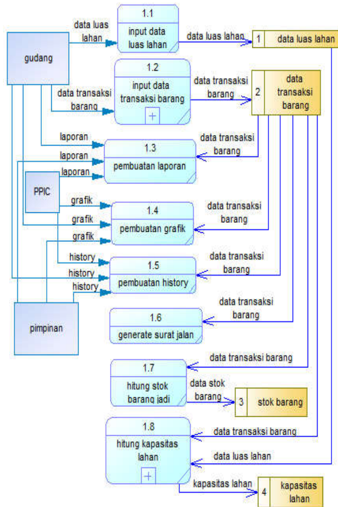
Figure 4 DFD Level 1
