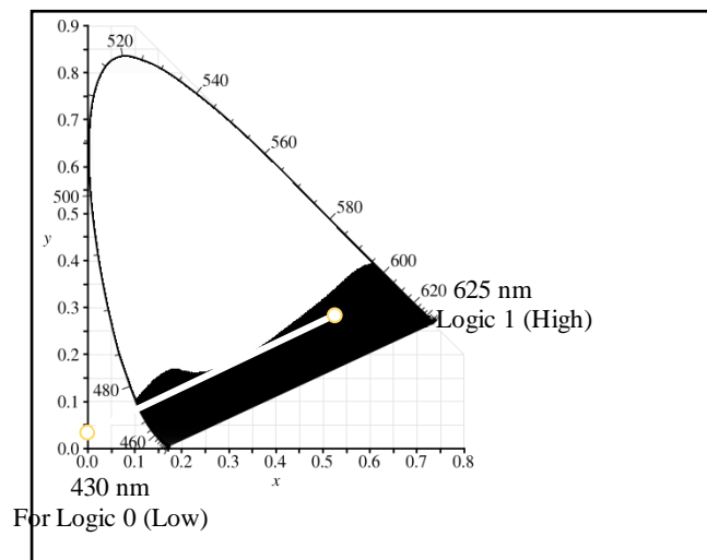
Figure 1. CIM Constellation Diagram
