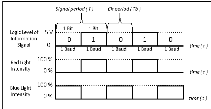
Figure 3. Line Coding Scenario
