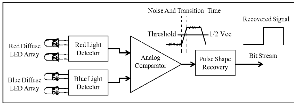
Figure 4. Complete VLC Demodulation System Design
