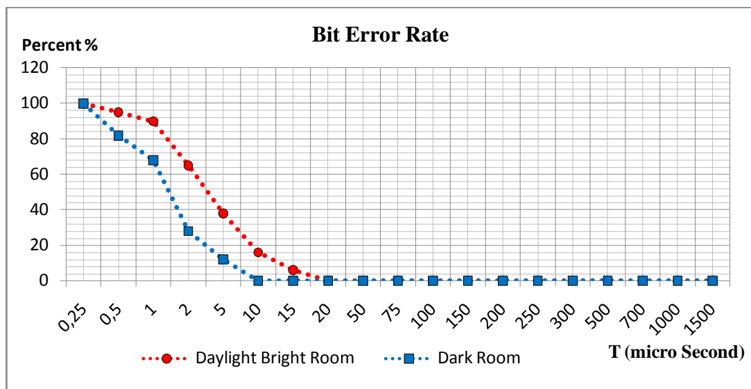
Figure 6. BER Trial Result
