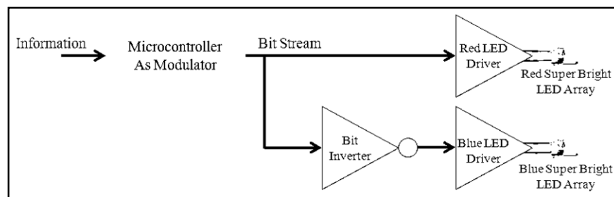
Figure 2. Complete VLC Modulation System Design
