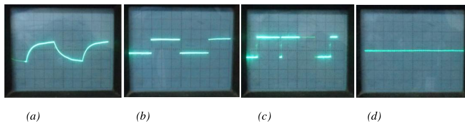
Figure 7.a. Pulse Shape Before Pulse Shape Recovery ( T \geq 20 \mu\text{s} ) Figure 7.b. Pulse Shape After Pulse Shape Recovery ( T \geq 20 \mu\text{s} ) Figure 7.c. Pulse Shape After Pulse Shape Recovery ( T = 10 \mu\text{s} ) Figure 7.d. Pulse Shape After Pulse Shape Recovery ( T \leq 1 \mu\text{s} )
