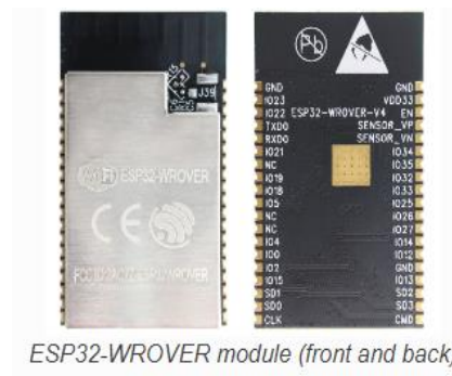
Figure 6. The ESP32-WROVER
