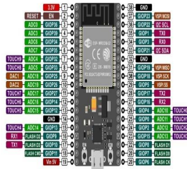
Figure 2. ESP32 Pinout Parts
