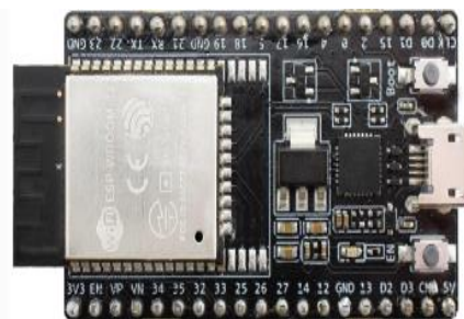
ESP32 DevKitC V4 board
